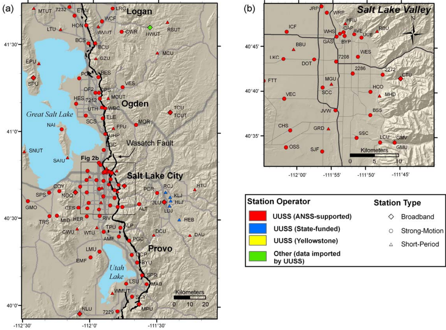
Figure 2. Real-time urban strong-motion network in the Wasatch Front urban corridor.
